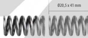
CC75043 Spring
