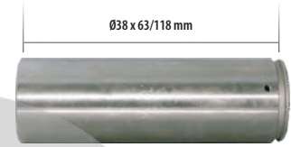
CC75081 Guide Pin (Long)
