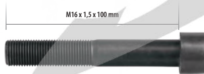
CC55007 Guide Pin Bolt (Long)
