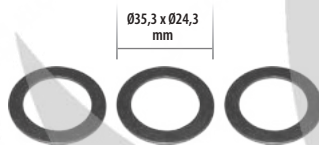
CC74098 Washer
