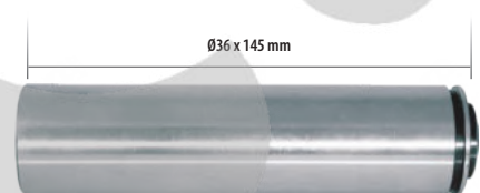
CC95003 Guide Pin (Long)
