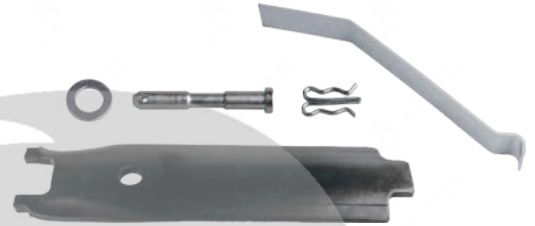
500-5813 Caliper Pad Retainer Repair Kit
