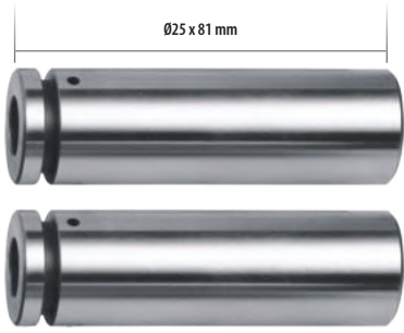
CC75005 Guide Pin (With Hole)
