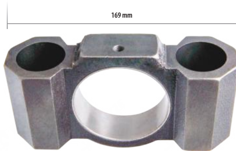
800-885-094 Caliper Bridge Assembly
