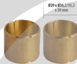
CC85085 Bronze Oval Bush
